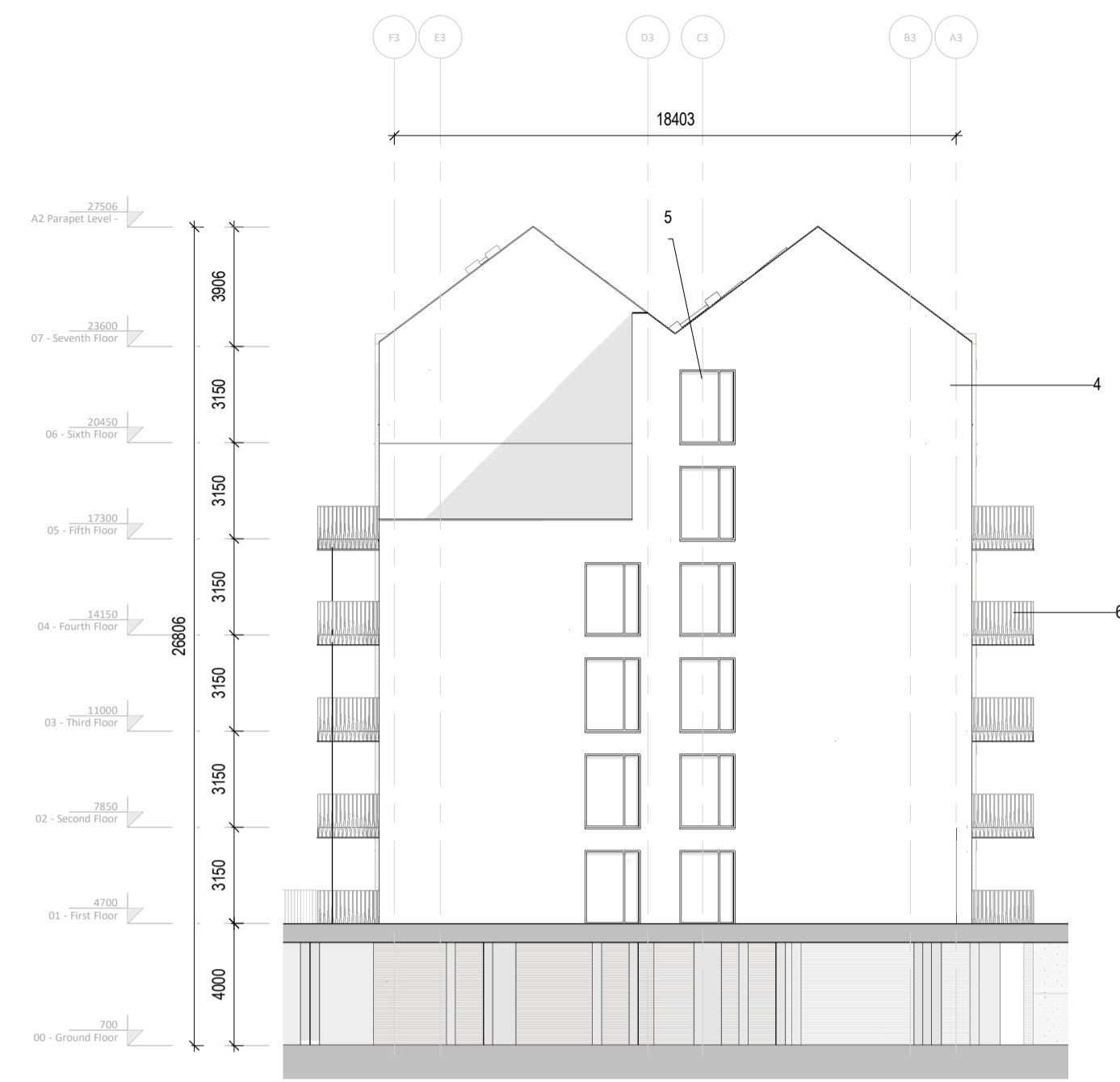
2 A3_North East Elevation 1:200
